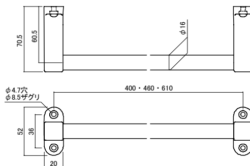
晾衣杆: \phi 16 mm
