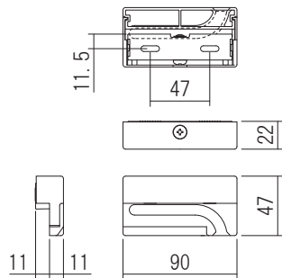
Spool Bracket (R)
