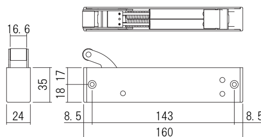
Soft Close for Sliding Door
