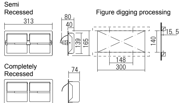
Completely Recessed
