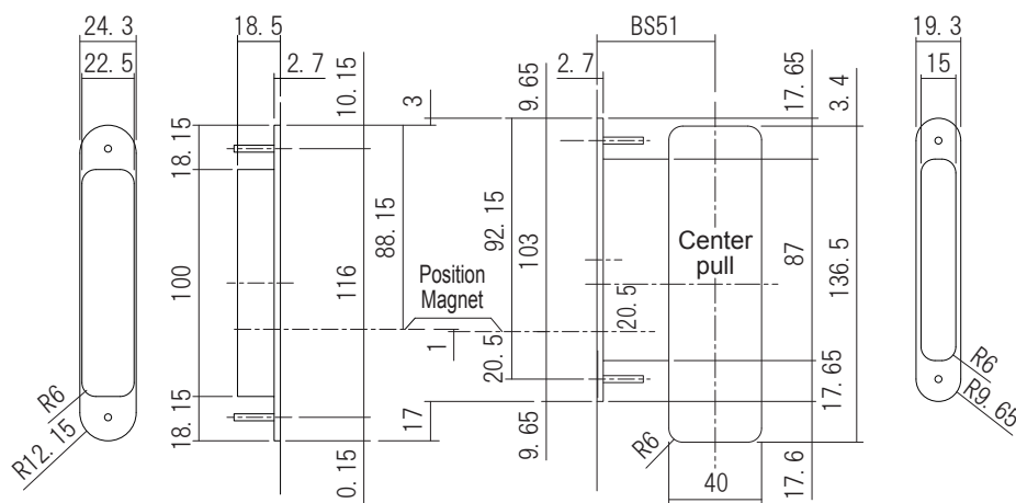
Figure drilling of strike
