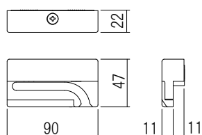
Bracket spool
