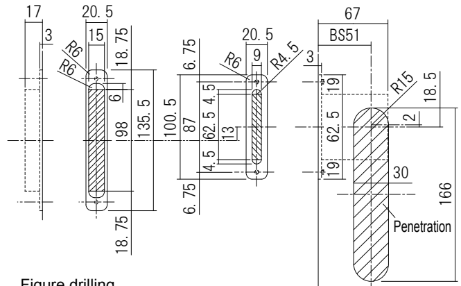
Figure drilling of strikes
