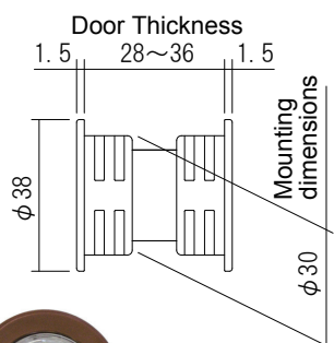
Lens of diamond cut specification(BK).
