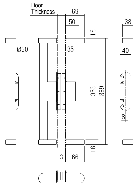
Both Side of Bar pull Specification
