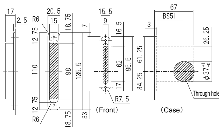
Figure drilling of strike
