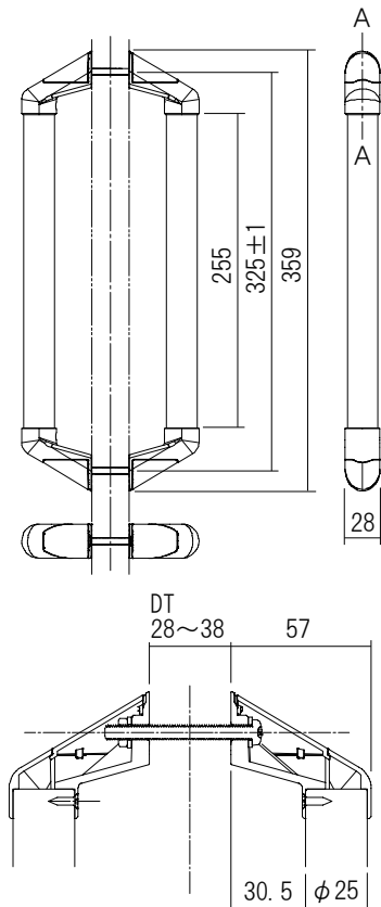
A-A Sections
