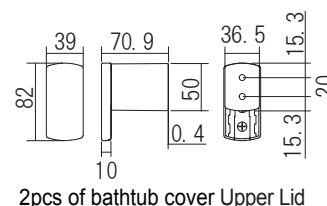
2pcs of bathtub cover Upper Lid
