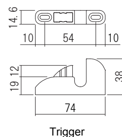
Soft Close for Sliding Door
