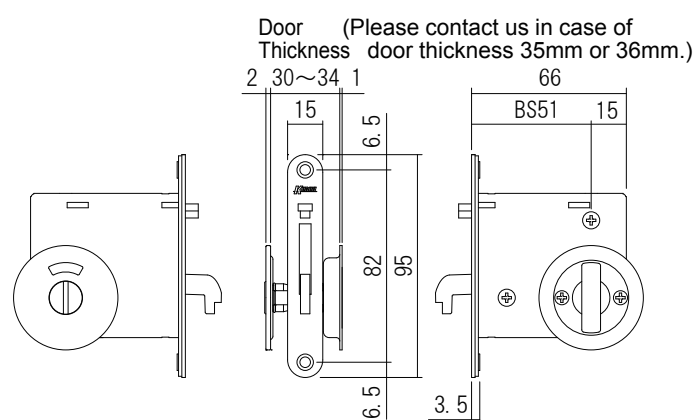
Clear Cut Hook Lock
