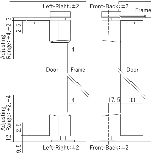
Drawing for Installation (Drawing for Right-Hand) ※ Digging is necessary on door and frame.
