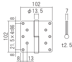
※ This drawing is Right-Hand
