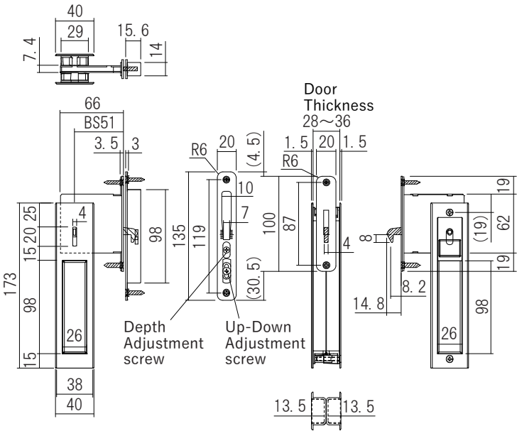
TS Hook Lock + Adjustment Strike
