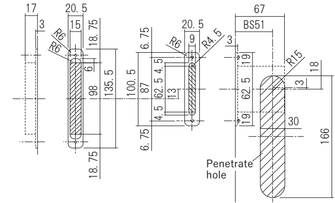
Strike digging drawing Pull-Lock Case digging drawing
