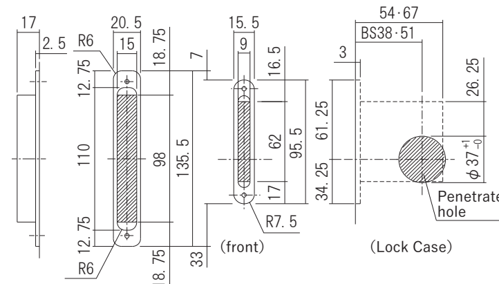
Lock Case digging drawing
