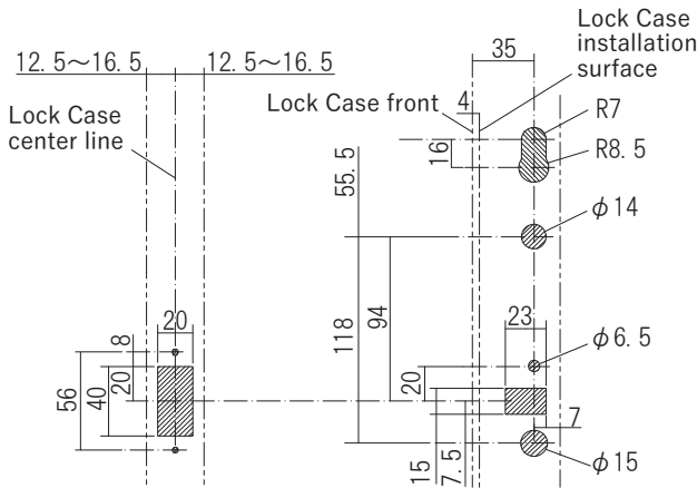
Cutaway view
