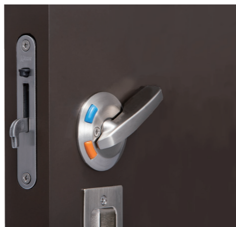
Dead Bolt Lock BS51 The hook lock strikes out from above. At the same time, the dead bolt protrudes. Back set is 51 mm.
