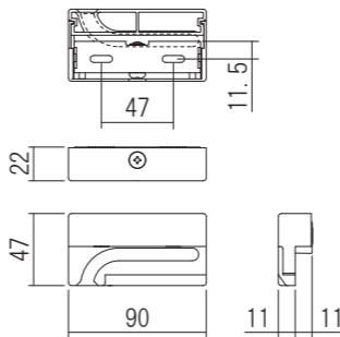
Spool Bracket (L)
