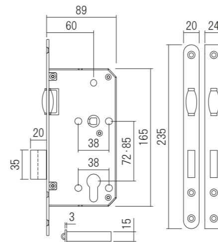
Roller lock
