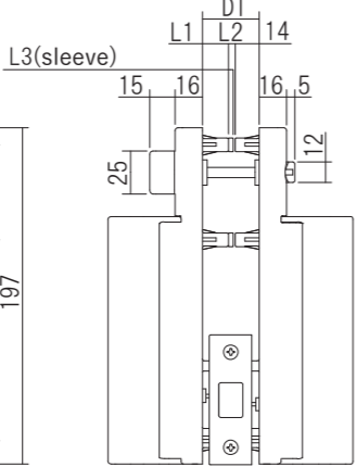
This drawing is for Right-Hand use.
