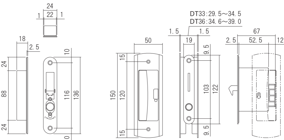
Adjustable Strike NS Automatic Hook Lock
