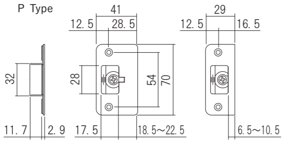
For small door
