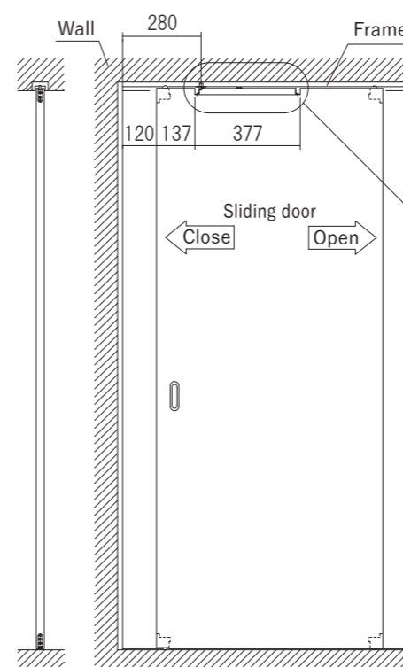
Drawing for Installation
