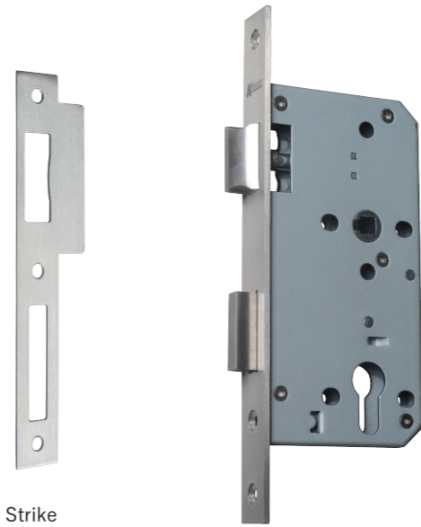
Sash Lock
