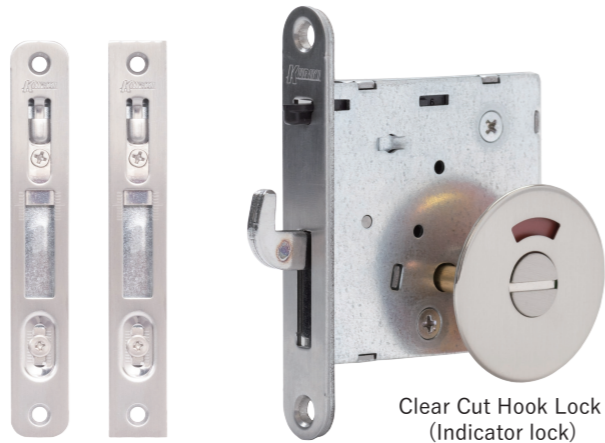
Bottom Lock BS51 The hook lock strikes out from the bottom. Back set is 51 mm.
