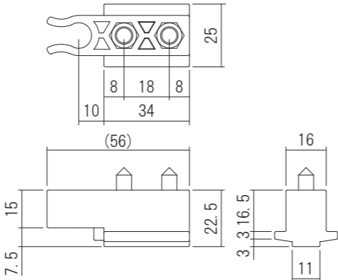
Upper Stopper
