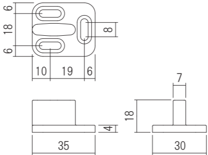
Floor Guide
