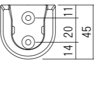
Bracket
