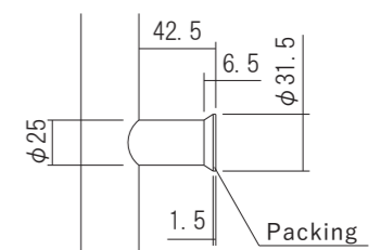
Specification of part a
