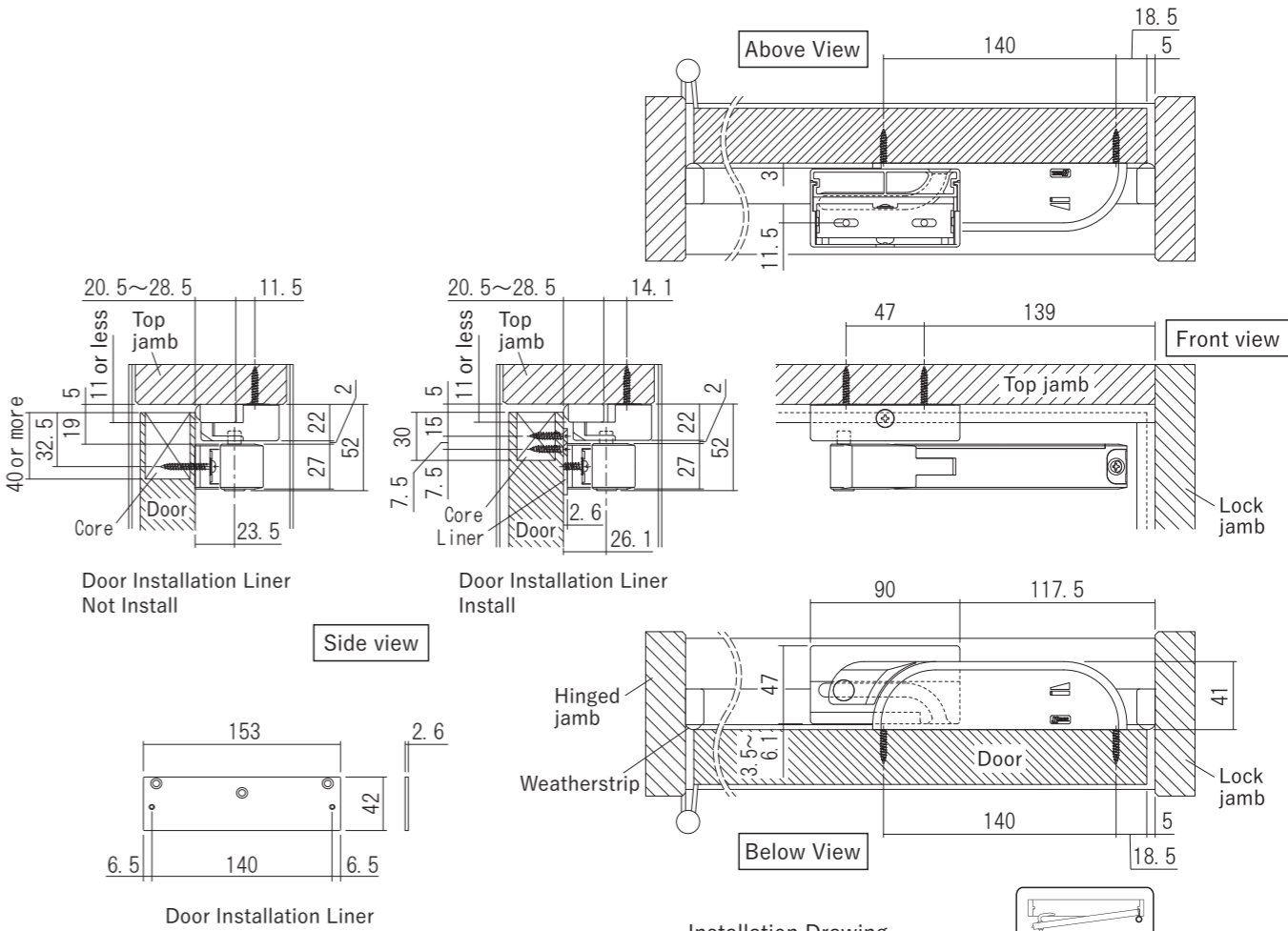
Installation Drawing (showing right hand opening)
