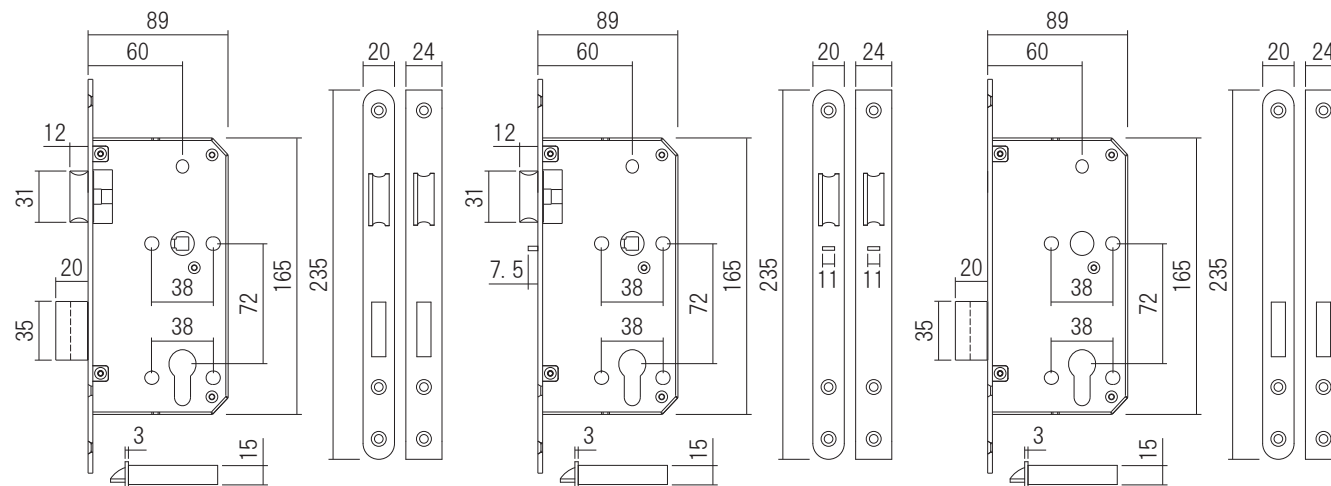
Sash lock
