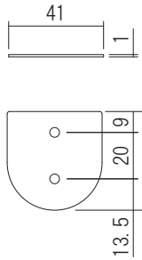
Base plate
