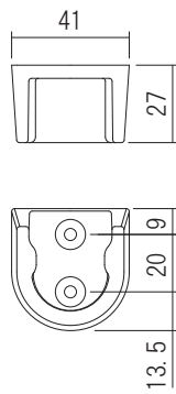
Bracket
