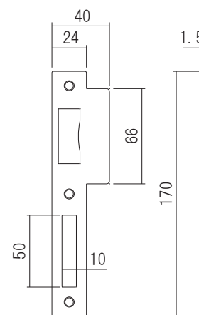
Strike
