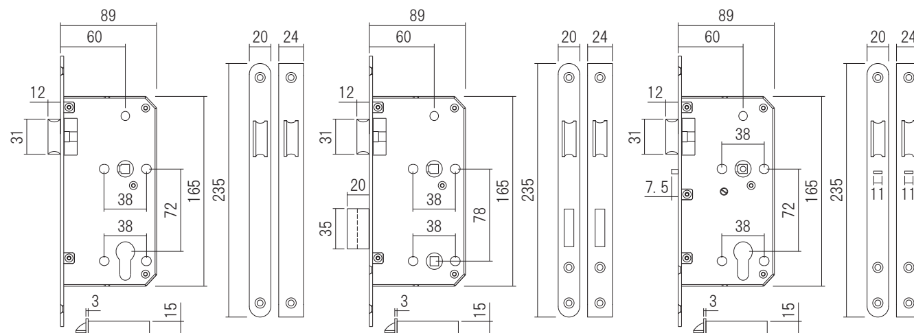
Passage lock
