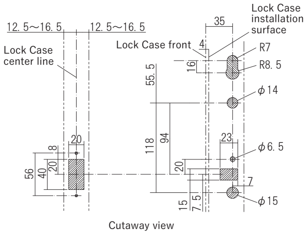
Cutaway view
