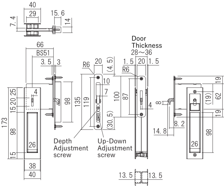
TS Hook Lock + Adjustable Strike
