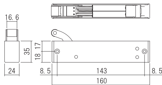
Soft Closer Main unit
