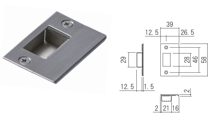
F Type
