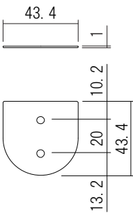
Base plate
