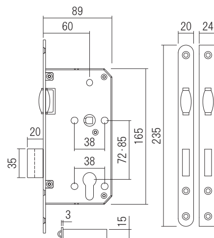
Roller lock
