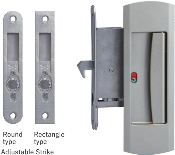
NS Automatic Hook Lock (Indicator lock)
