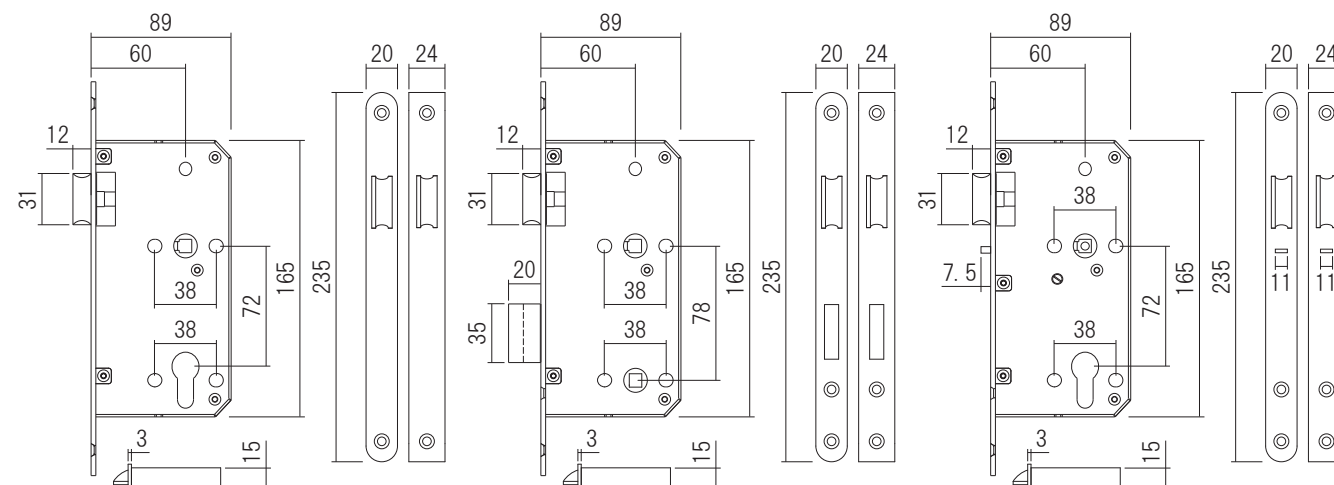
Passage lock
