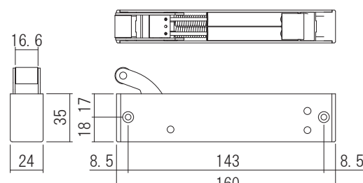
Soft Closer Main unit
