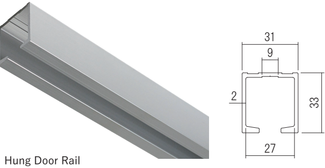
Hung Door Rail
