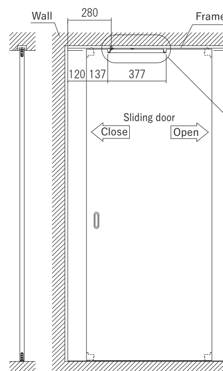
Drawing for Installation
